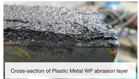
WP - sag mill chute liner repair & wear protection
